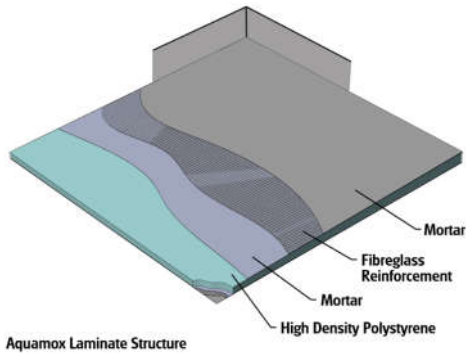
Aquamox Laminate Structure
